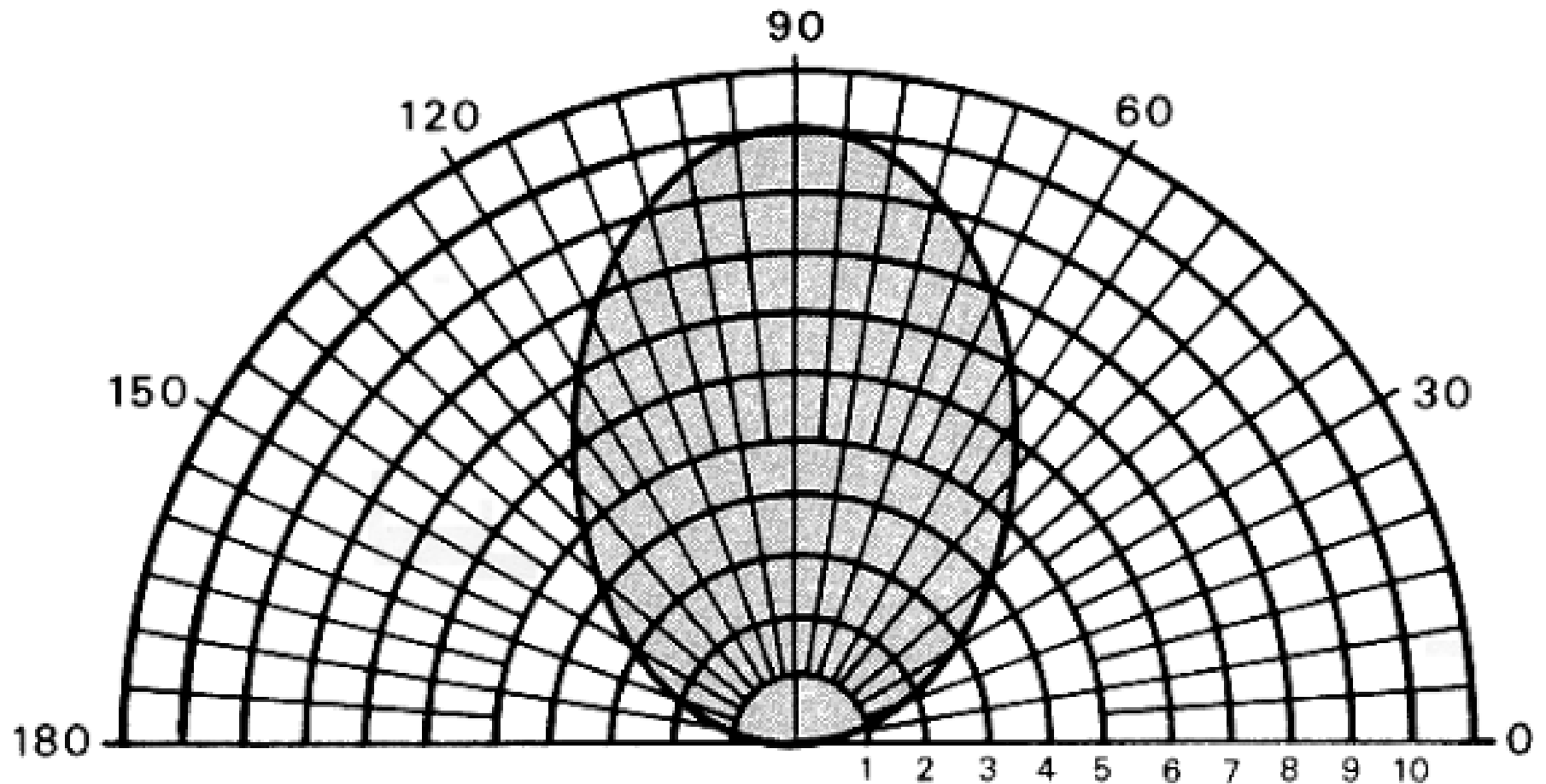
Figure M-6 Typical elevation plane patterns for half-wavelength antennas one-eighth wavelength or less above ground.
